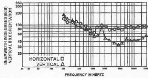
FIGURE 5 — MTH-2.5/94BT Directivity vs. Frequency
