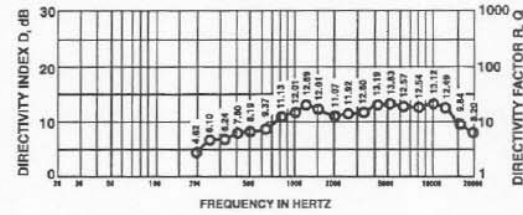
FIGURE 5 — MTH-2.5/94BT Directivity vs. Frequency
