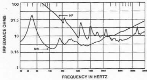
FIGURE 2 — MTH-2.5/94BT Impedance vs. Frequency
