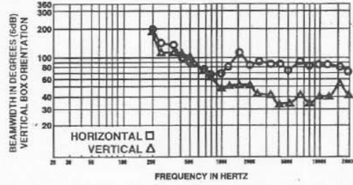
FIGURE 4 — MTH-2.5/94BT Beamwidth vs. Frequency
