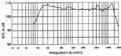
FIGURE 1 — MTH-2.5/94BT Axial Frequency Response
