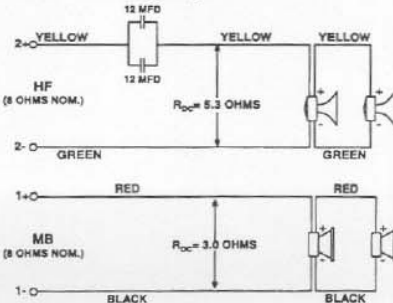
FIGURE 7 — MTH-2.5/94BT Wiring Diagram
